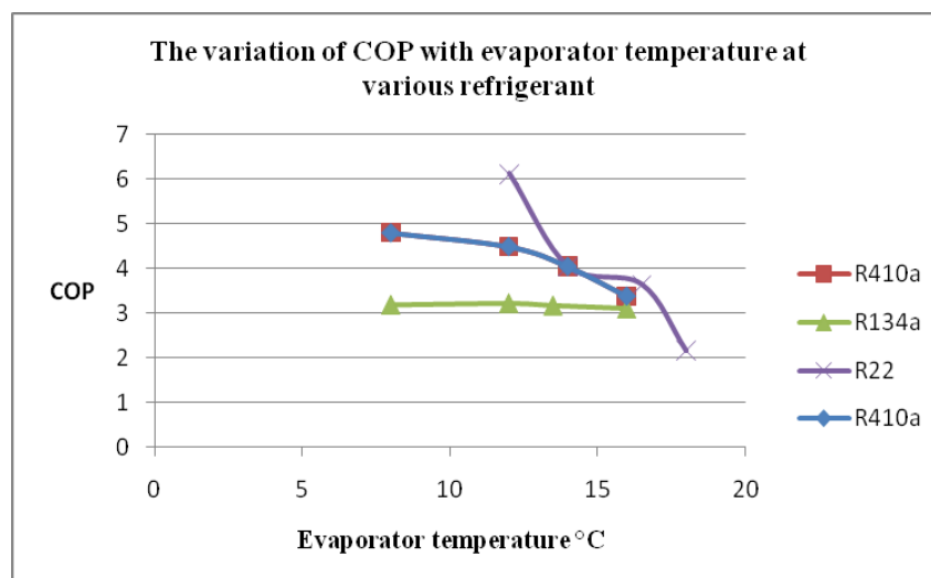
Figure 2: Graph of COP VS Evaporator temperature for various refrigerants
